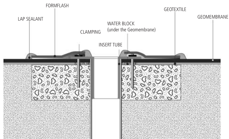
Fig. 24 : Water discharge with insert pipe
