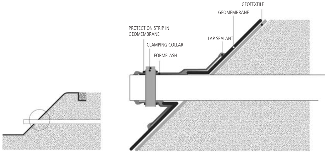
Fig. 22 : Mechanical Securement with clamping collar
